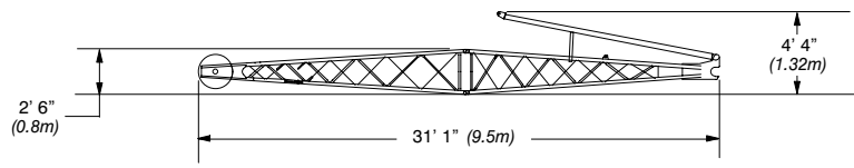
Carbody Jack minimum and maximum heights
