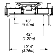
Carbody Jack minimum and maximum heights
