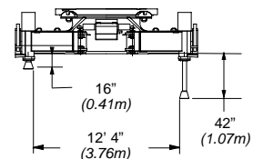
Carbody Jack minimum and maximum heights 16, 992 lbs. (7 707 kg)
