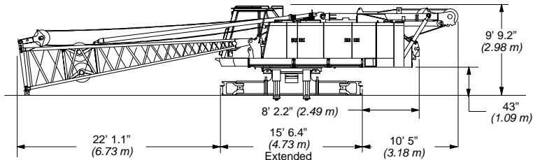
Upper & Carbody Shipping Weight Rope on both drums, backstops, catwalks, and full tank of fuel 85,158 lbs. (38 627 kg)
