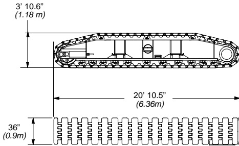
Tread Members w/36" (0.9 m) Shoes 23,543 lbs. (10 679 kg) – each
