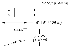
Right Wing Counterweight 6,615 lbs. (3 001 kg)
