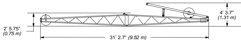
30' (9.1 m) Basic Jib Assembly- Tube: 1,676 lbs. (760 kg)
