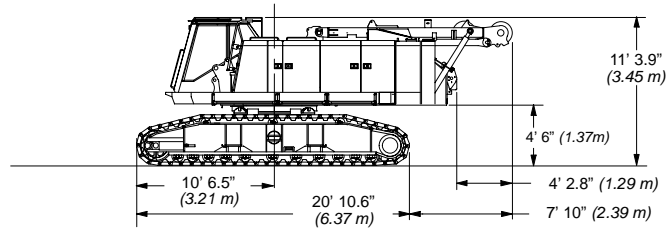
Transport Weight Rope on both drums, Treadmembers Backstops, Catwalks and full tank of fuel 118,329 lbs. (53 673 kg)
