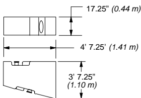
Left Wing Counterweight 6,836 lbs. (3 101 kg)
